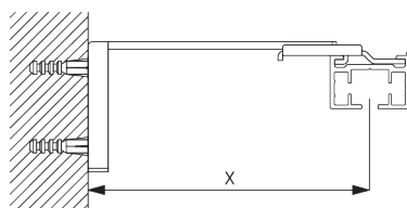
Smart Fix SG 11200 - SG 11205 and bracket SG 3041: Screw SG 10492 (M4x8) needed.
